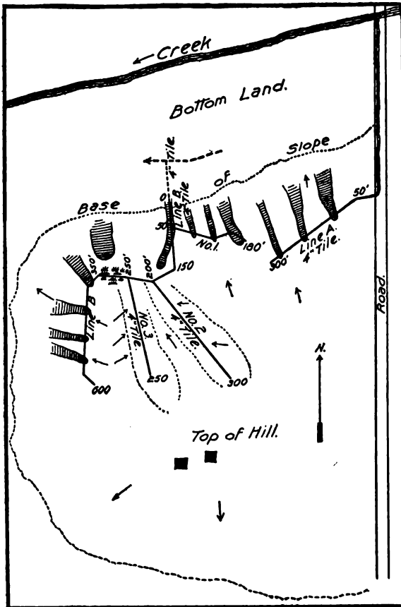
FIG. 122.—Plan of underdrains for Georgia hillside experiment.
