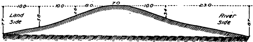
FIG. 110.—Hunt district levee—section of new levee built to cross crevasse.
