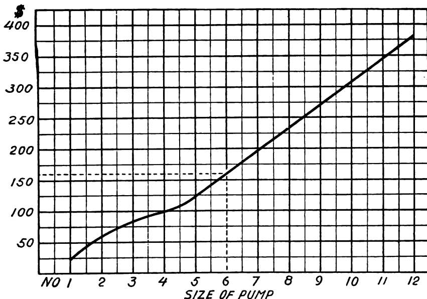
FIG. 32.—Approximate cost of centrifugal pumps.
