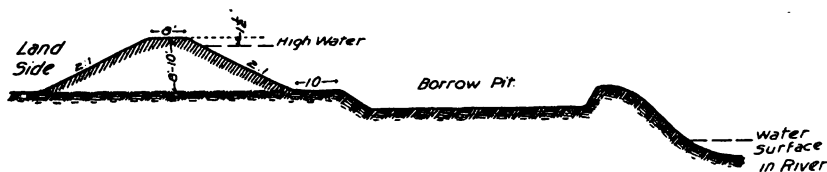
FIG. 90.—Specified section of Sugar Creek levee.
