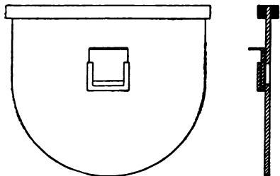
FIG. 65.—Regulating gate for laterals.
