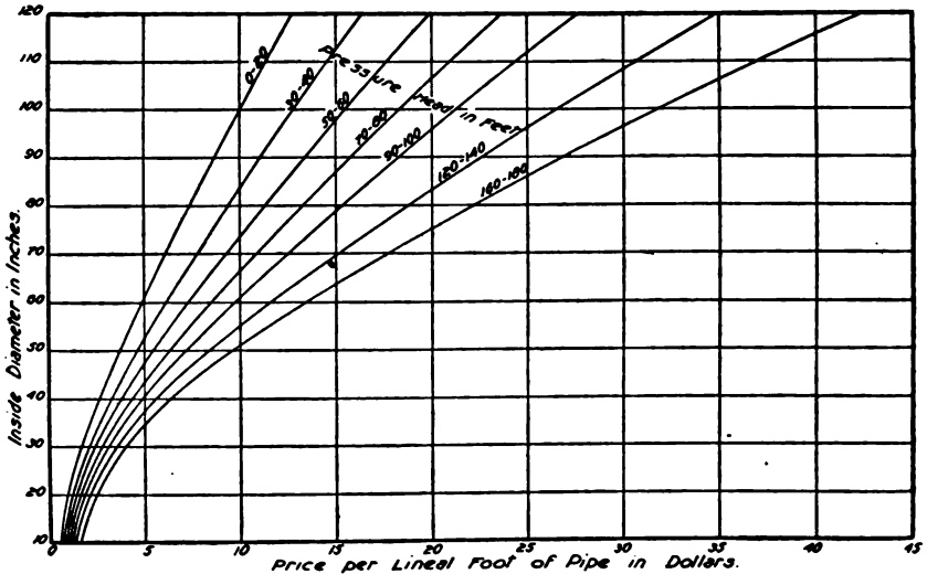
FIG. 55.—Cost of wooden stave pipe.
