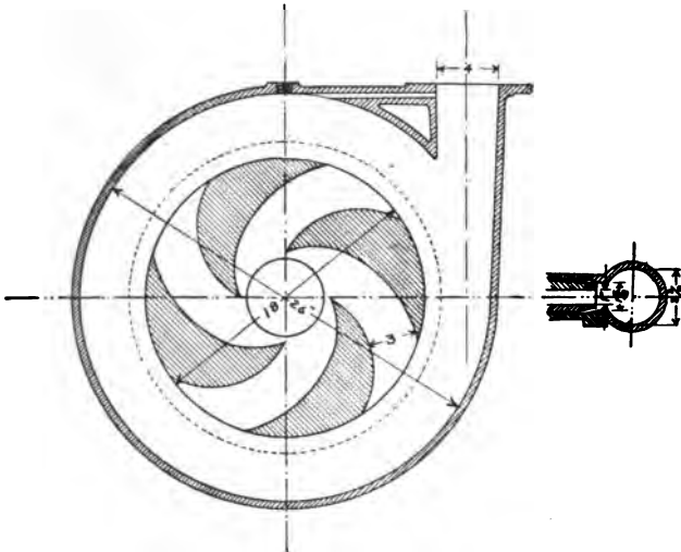
FIG. 25.—Section of pump used in test No. 5.
