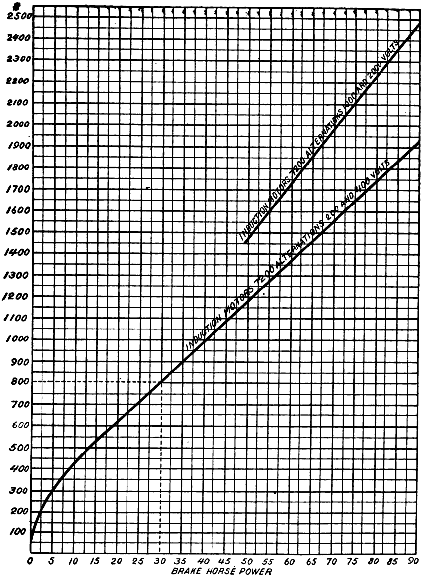
FIG. 35.—Approximate cost of induction motors.
