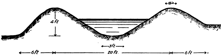
FIG. 6.—Cross section of well-made laterals.
