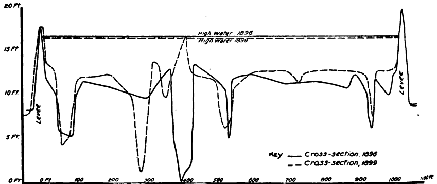
FIG. 105.—Section across Bear Creek waterway.
