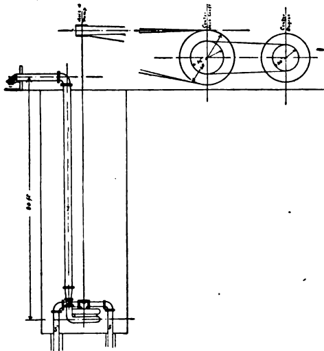
FIG. 9.—Plan of pumping plant owned by William Bogen.
