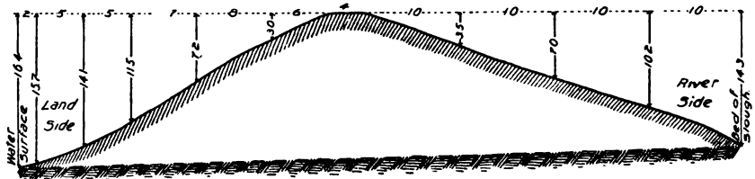
FIG. 99.—Flint Creek-Iowa River levee—section at northern part of Ziegler's Slough, sloughed in 1908.
