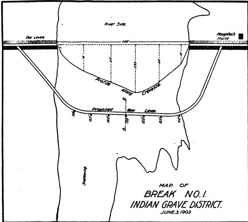
Fig. 116.—Map of break No. 1, Indian Grave district.
