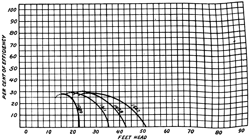
FIG. 22.—Efficiency curves, test No. 3.
