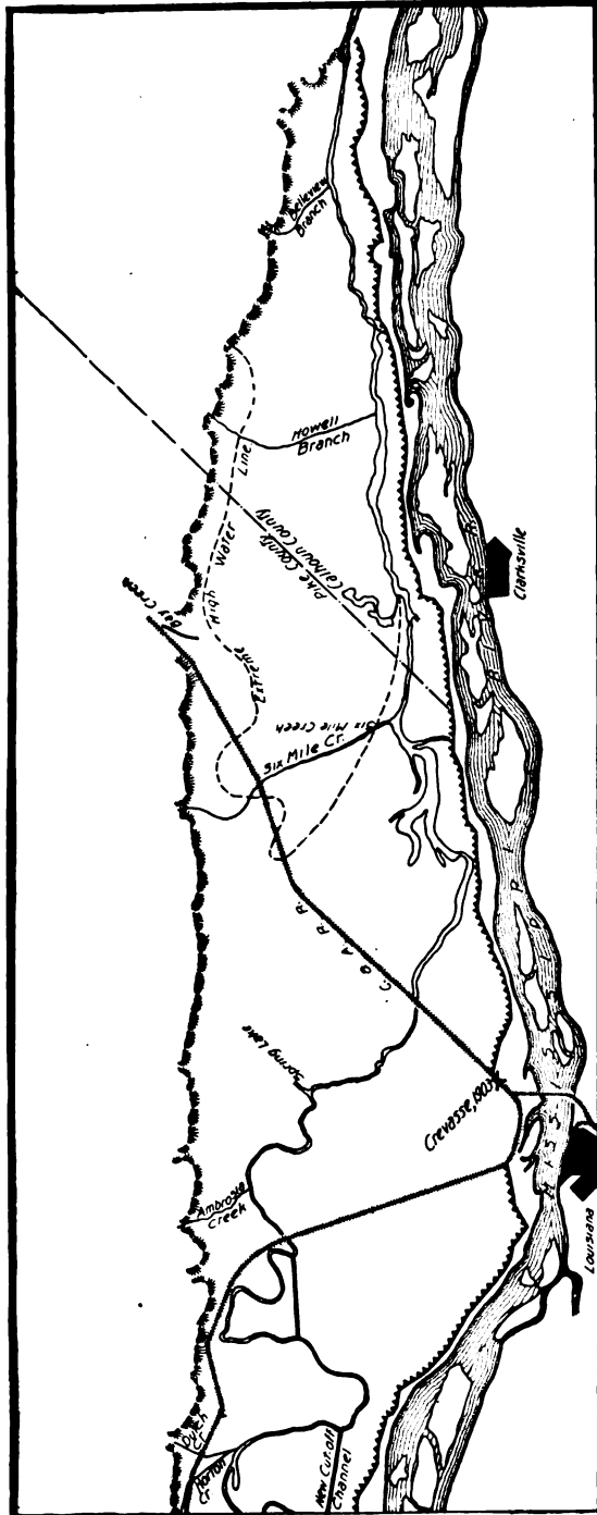
FIG. 107.—Map of a part of Sny Island levee and drainage district.
