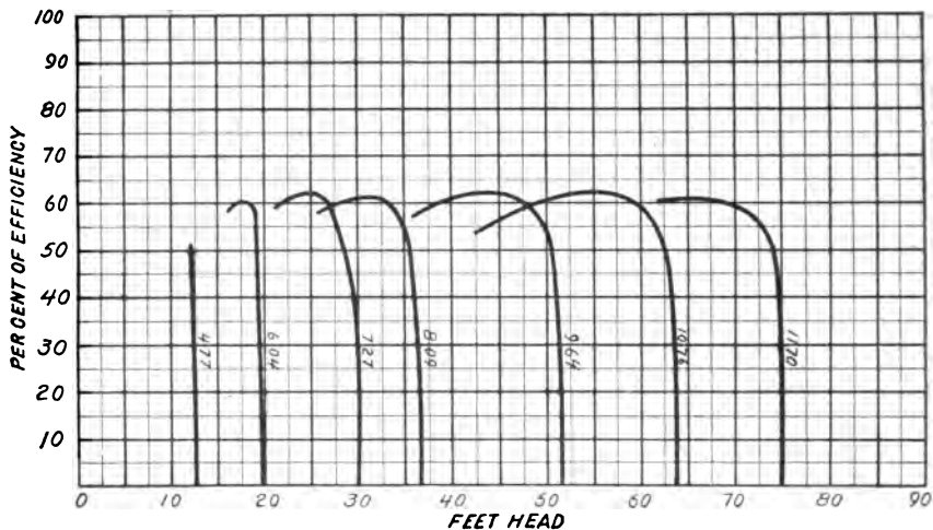
FIG. 20.—Efficiency curves, test No. 1.
