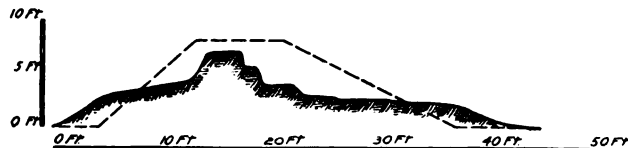
FIG. 87.—Lacey district—change in section of levee since first constructed.
