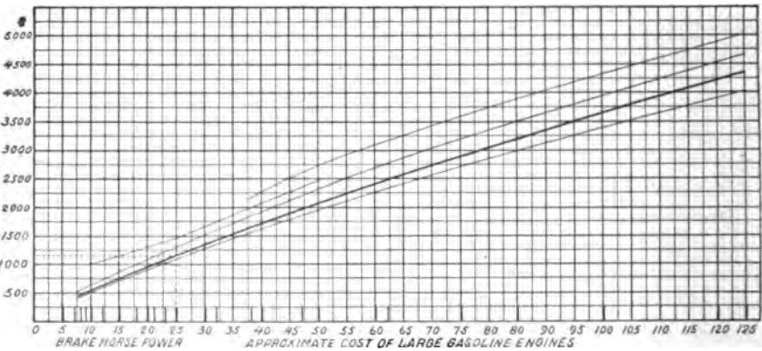
FIG. 34.—Approximate cost of large gasoline engines.
