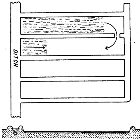
FIG. 61.—Bed Irrigation.
